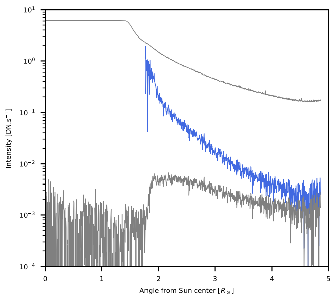
Fig. 5. Raw (lower gray) and vignetting-calibrated (blue) radial 17.4 nm intensity profiles, averaged over the sector shown in Fig. 3. The top curve corresponds to the data taken without the occulter disk.
