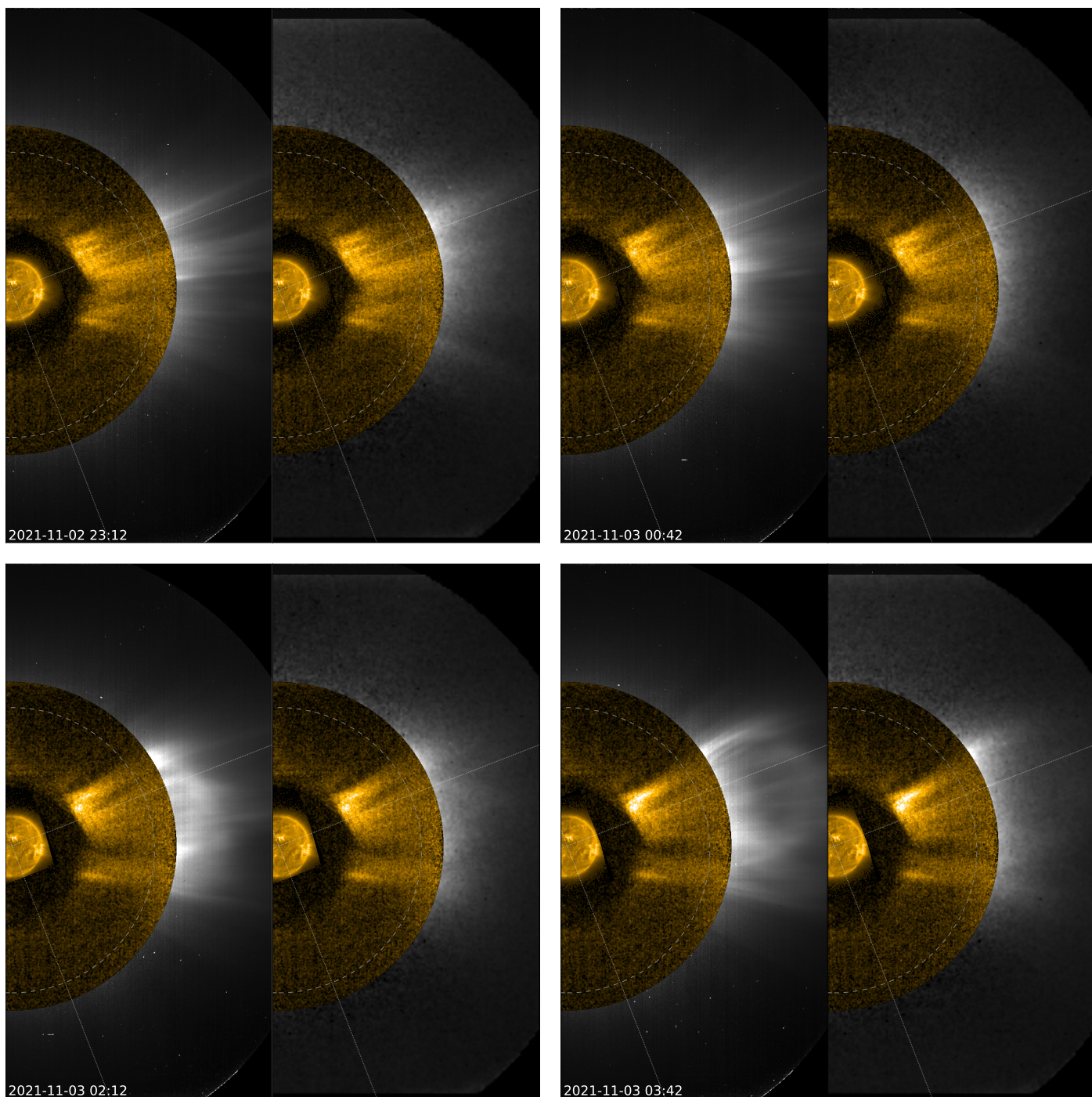
Fig. 8. Propagation of a CME across the FSI and Metis FOVs . Left and right sides of each panel show a comparison of SWAP (below 2 R_{\odot} ) and FSI 17.4 nm (up to 5.6 R_{\odot} ) with Metis VL and Lyman \alpha data, respectively. The dashed circle marks the position of the edge of the Metis occulting disk. An animated version of the figure is available online.
