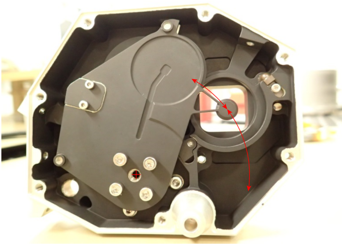
Fig. 4. Entrance door of FSI, looking towards the Sun. The occulter disk is held off the door lid by two supporting rods. The occulter disk is shown in position. Rotating the lid around its axis (red cross) clockwise closes the door, rotating it counter-clockwise opens it.
