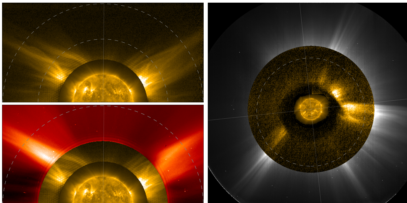
Fig. 11. Comparison of the northern half of the overlapping region between FSI and LASCO C2 on 2022 March 7. Top: FSI composite (same images as in Fig. 10), extending to the edges of the detector. The outer dashed circle corresponds to the 3.4 R_{\odot} boundary between FSI and LASCO C2 used in Fig. 10. The inner dashed circle corresponds to the boundary between FSI and LASCO C2 used in the bottom panel. Bottom: Same as above, with LASCO C2 above 2.2 R_{\odot} , the inner limit of the useful LASCO C2 FOV.
